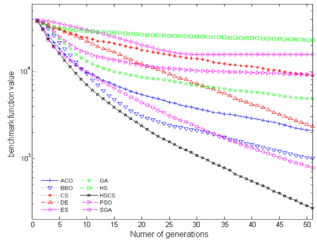
Fig. 11 Fitness curves of ten methods for the F14 function
