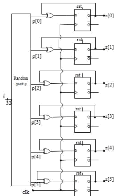
Fig 3: Output bits Encoding
