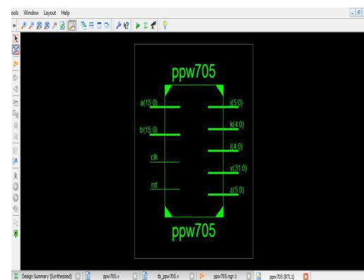
Fig 10: RTL Design of Main project work
