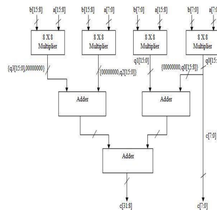
Fig2 : 16-bit X 16-bit Multiplier
