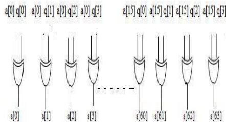
Fig 4: 64-bit Encryption key generator
