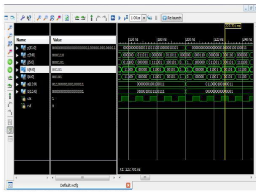
Fig 9: Simulation result of main project work
