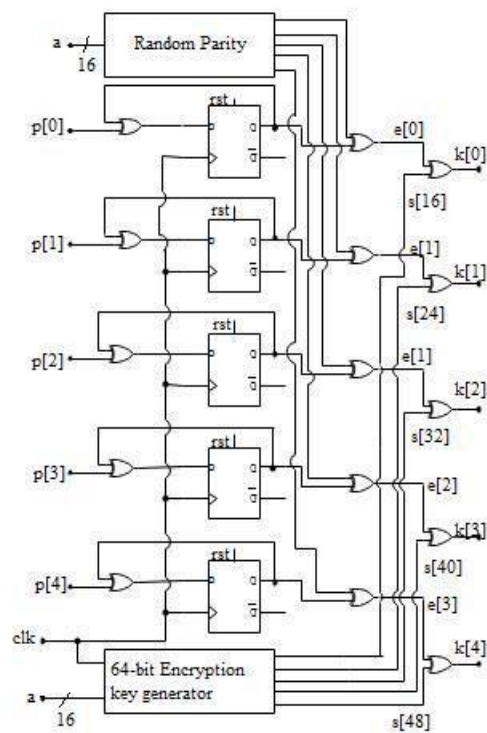
Fig 5: Input bits Decoding
