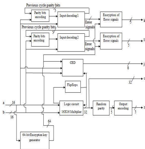
Fig 1: Main Project work Architecture
