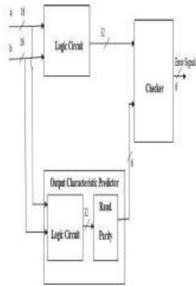
Fig 6: Concurrent Error Detection (CED)
