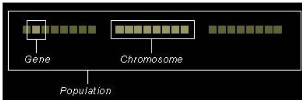
Fig 1: GA Population [13]
