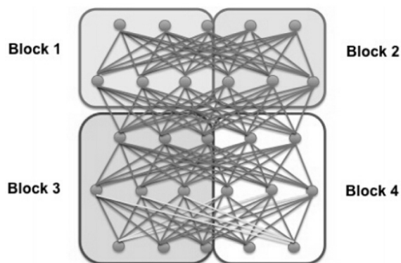
Fig. 10. Example of DistBelief with four blocks.
