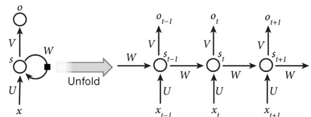
Fig. 8. Recurrent neural network.
