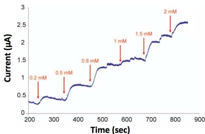
Fig. 7. Continuous monitoring with the single-metabolite remote system and a lactate bio-nano-sensor.
