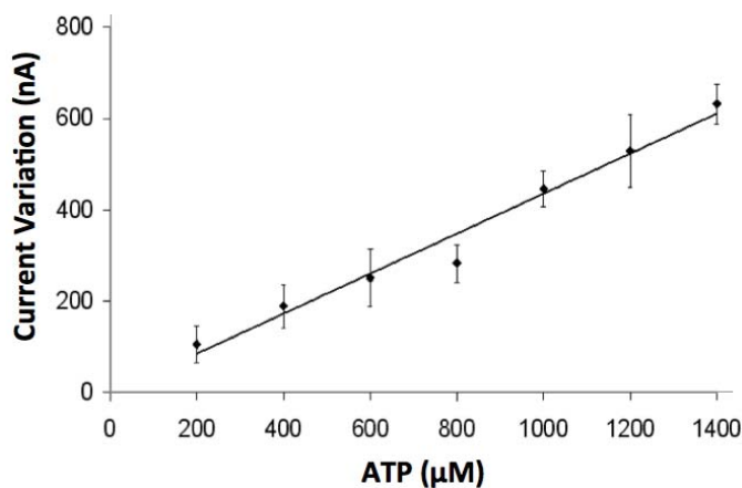
Fig. 5. Calibration curve for ATP detection in the 0 to 1.4 mM concentration range.
