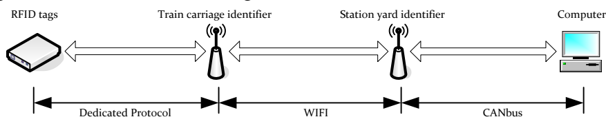
FIG. 2. Electronic recognition mode
