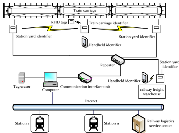
FIG. 1. Constitution of the electronic recognition system
