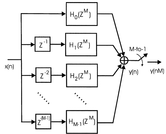
Fig. 21. M -path partition of prototype low-pass filter with output resampler.
