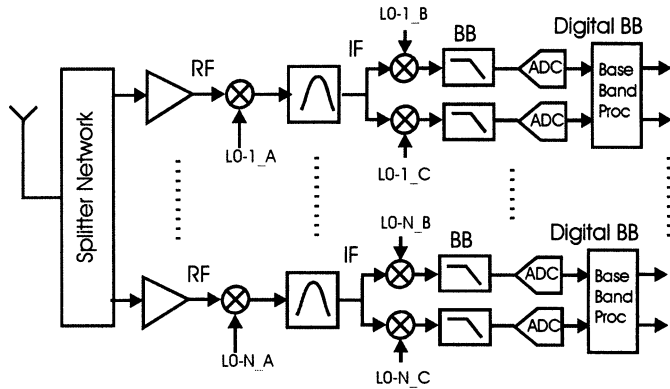
Fig. 1. First-generation RF architecture of N -channel receiver.
