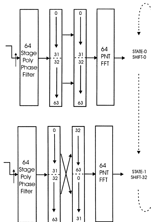
Fig. 30. Cyclic shift of input data to FFT to absorb phase shift due to linear time shift of data through polyphase filter.
