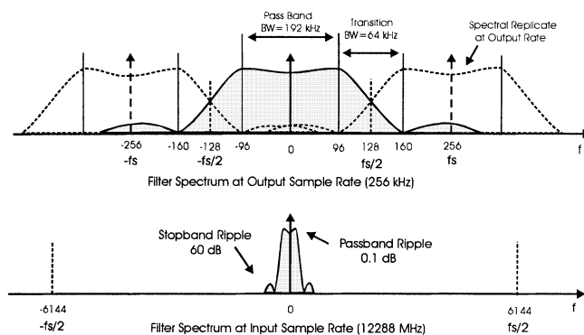
Fig. 35. Spectral characteristics of prototype filter at output and input sample rates.
