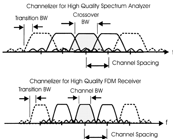
Fig. 28. Spectral characteristics of two channelizers with same channel spacing one for spectral analysis and one for FDM channel separation.
