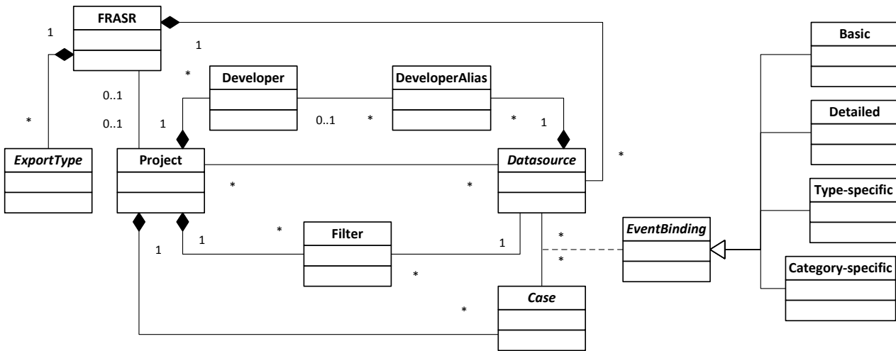
Figure 2. Architecture of FRASR
