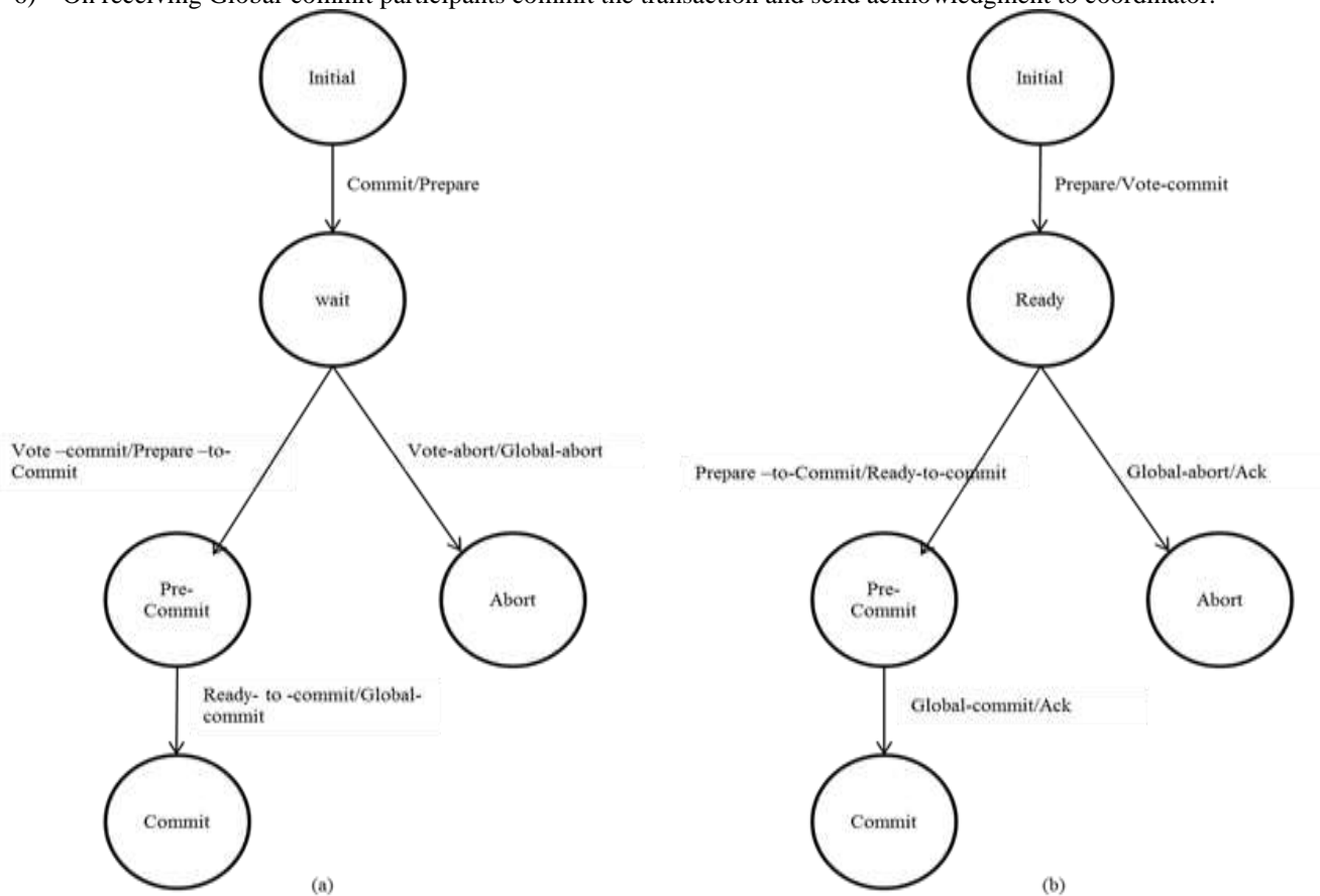
Fig. 4: State transition of (a) Coordinator (b) participant in 3PC [8]
