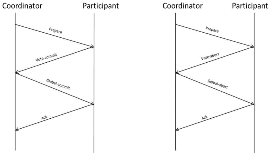
Fig. 2: Two-phase commit process
