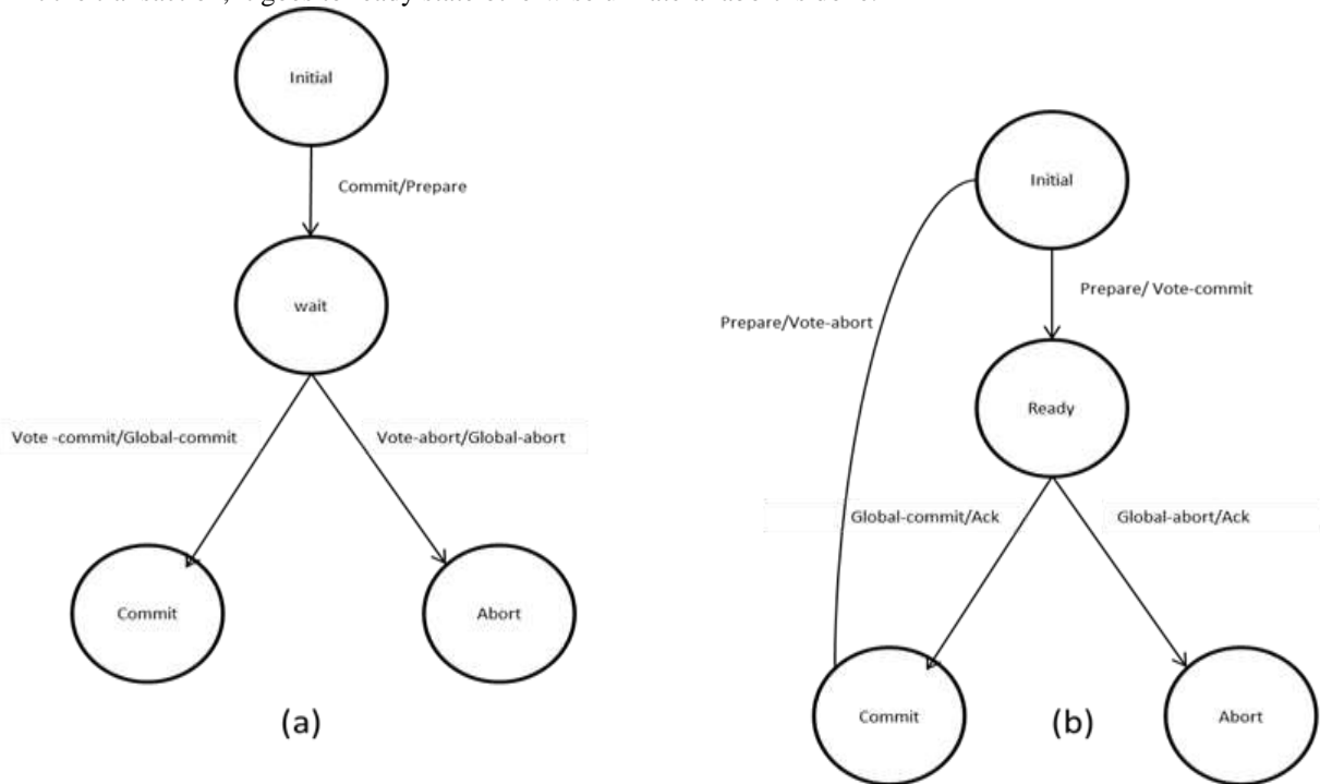
Fig. 3: State transition of (a) Coordinator (b) participant in 2PC [8]
