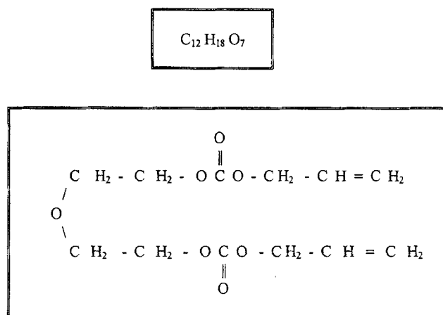
FIGURE 3 Chemical Structure of PADC.
