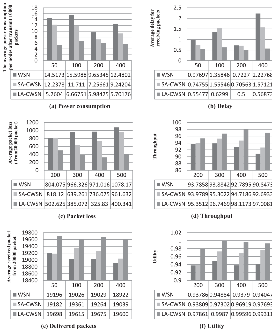
Fig. 5. Comparison the performance of LA-CWSN with SA-CWSN and the basic WSN (the charts are obtained by conducting several experiments at random starting parameter configurations and then averaging over these results is done.)
