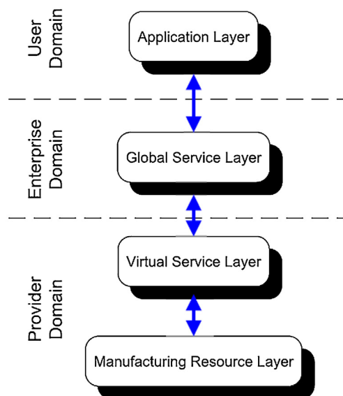
Fig. 7. CM layered framework, from [6].
