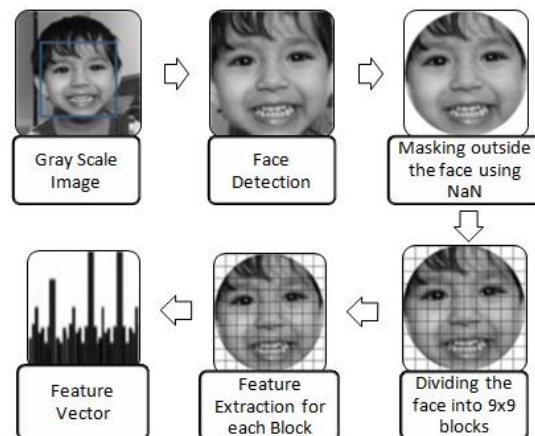
Fig. 6: Facial Feature Extraction
