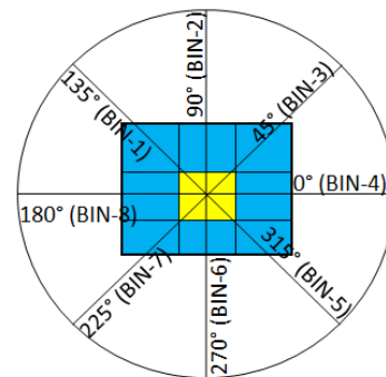
Fig. 4: 8 possible BINS denoted as 0°, 45°, 90°, 135°, 180°, 225°, 270° and 315°
