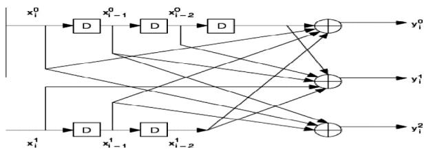
Figure 4 Convolutional Encoder.
