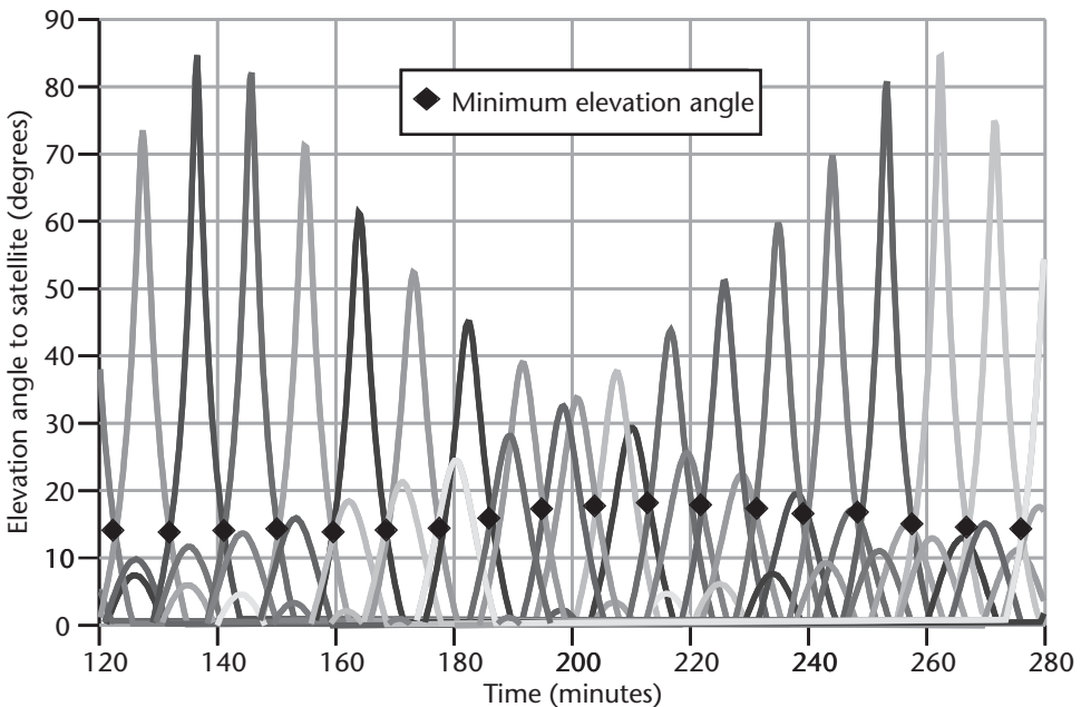
Figure 11.21 Iridium coverage at 55 NL (66 satellites, 86.4° inclination, 785-km altitude). (Courtesy of David Bell.)
