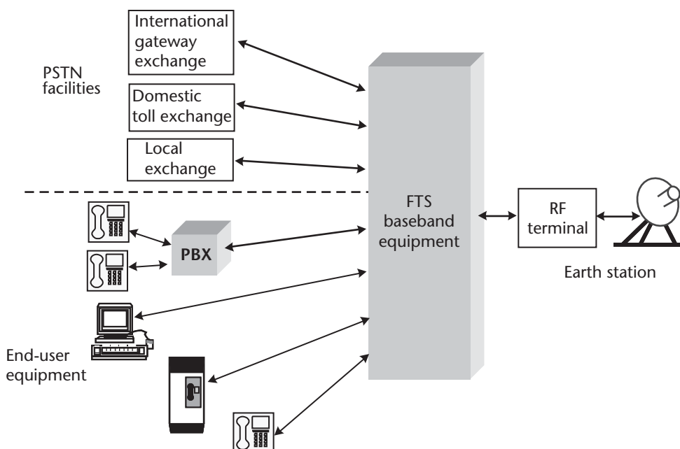
Figure 10.9 The range of interfaces to be employed in FTS applications, considering the connection to user devices as well as various options for the interface to the PSTN.
