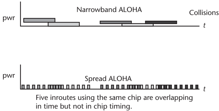
Figure 9.7 Application of CDMA in spread ALOHA to inbound multiple access. Narrowband ALOHA cannot support high throughput, as illustrated in the upper timeline. Overlap in time, as shown for Spread ALOHA does not result in collision unless chip sequence aligns in time. (Courtesy of Aloha Networks.)
