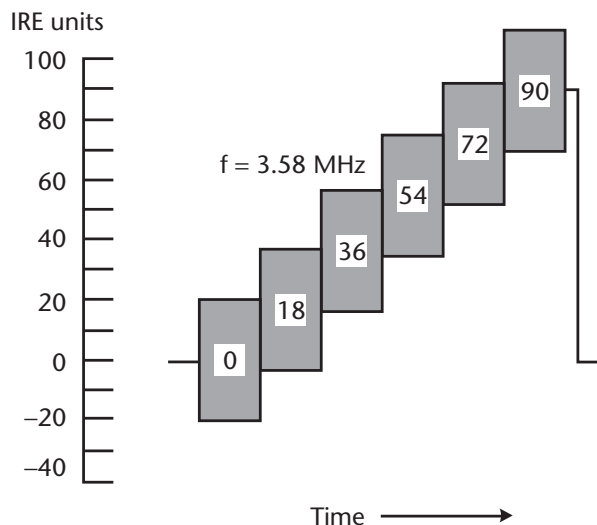
Figure 4.14 The modulated stairstep signal used to measure amplitude and phase nonlinearity as part of EIA/TIA 250-C testing.
